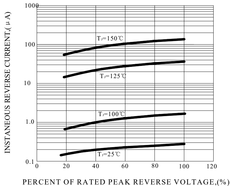
FIG.5-TYPICAL REVERSE CHARACTERISTICS
