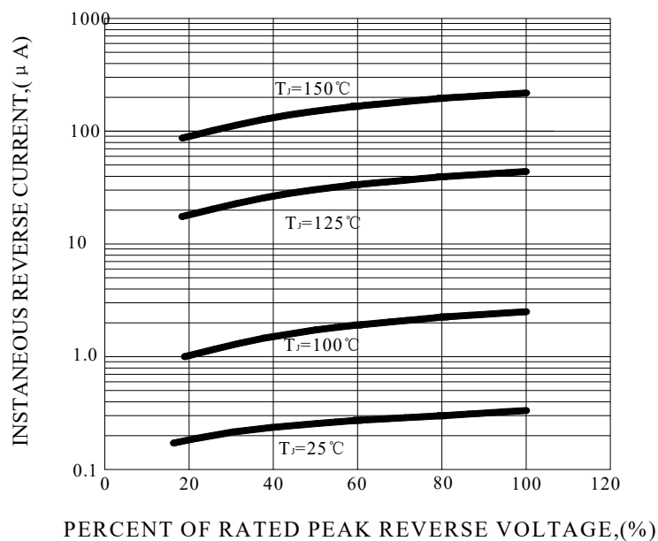
FIG.5-TYPICAL REVERSE CHARACTERISTICS
