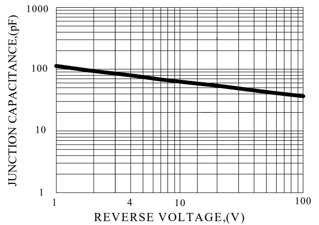
FIG.4-TYPICAL JUNCTION CAPAOTANCE
