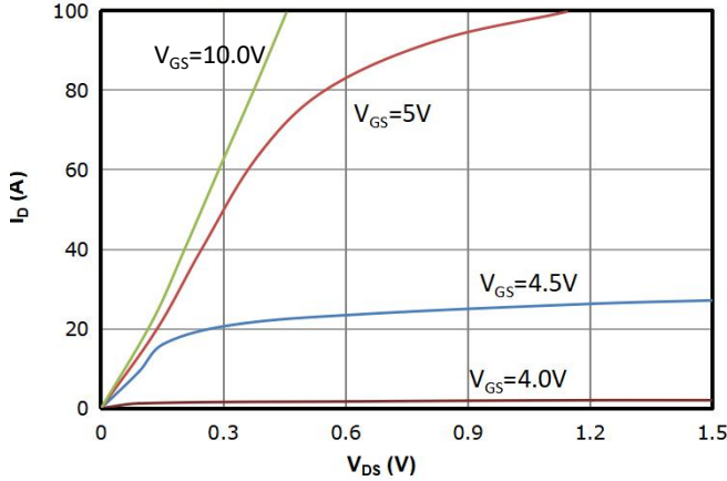
Fig 1: Output Characteristics
