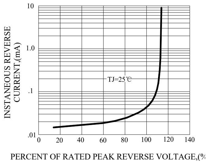
FIG.4-TYPICAL REVERSE CHARACTERISTICS
