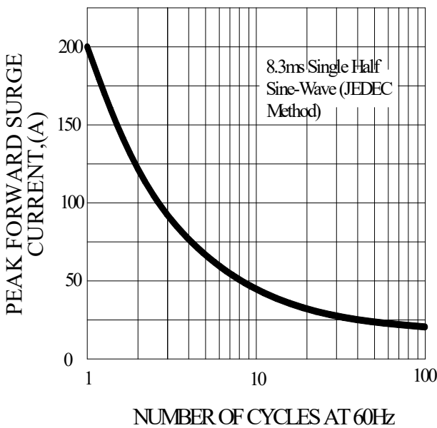
FIG.3-MAXIMUM NON-REPETTITIVE FORWARD SURGE CURRENT
