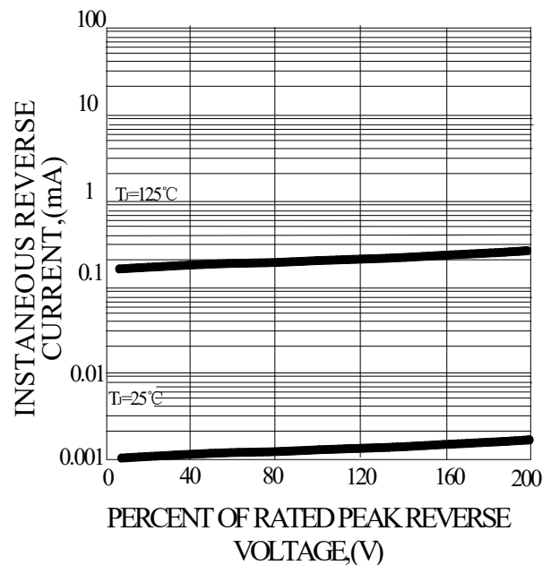
FIG.4-TYPICAL REVERSE CHARACTERISTICS
