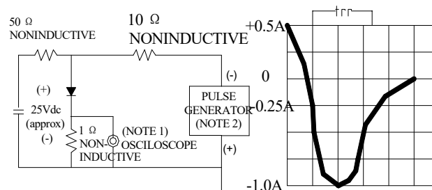
FIG.5-TEST CIRCUIT DIAGRAM AND REVERSE RECOVERY TIME CHARACTERISTIC
