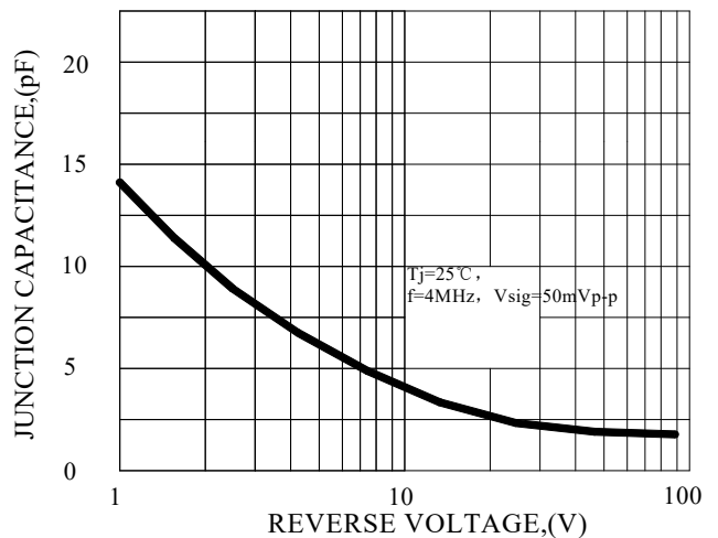
FIG.6-TYPICAL JUNCTION CAPACITANCE
