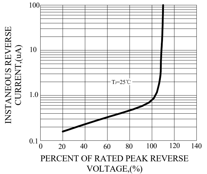
FIG.4-TYPICAL REVERSE CHARACTERISTICS
