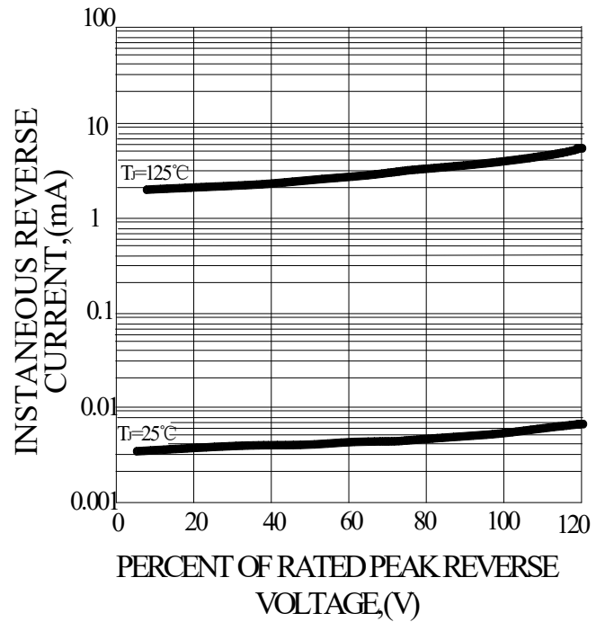
FIG.4-TYPICAL REVERSE CHARACTERISTICS
