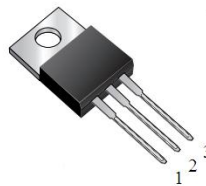
TO-220AB-3L PS40U120CT
