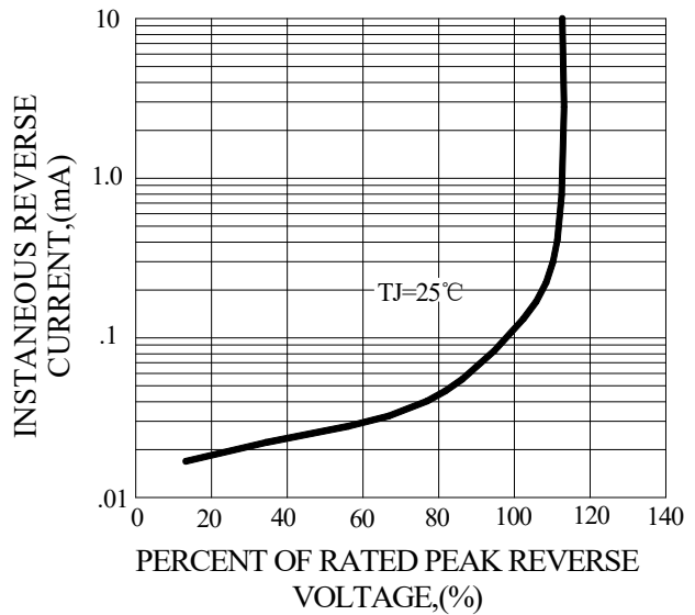
FIG.4-TYPICAL REVERSE CHARACTERISTICS
