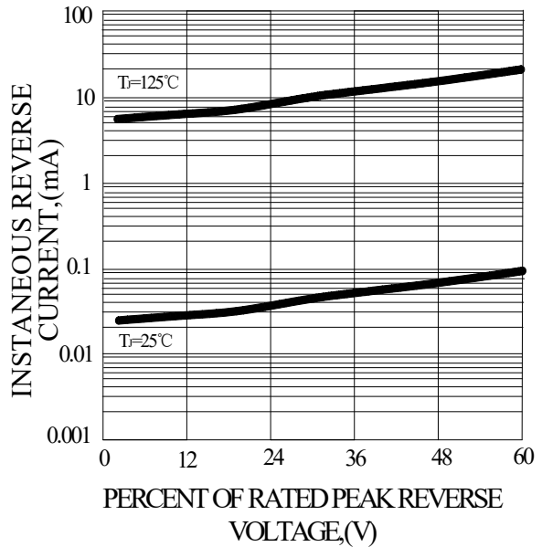
FIG.4-TYPICAL REVERSE CHARACTERISTICS
